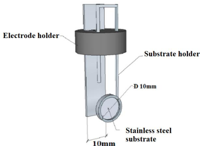
Figure 2.3. Two-electrode system designed for electrophoretic deposition.
