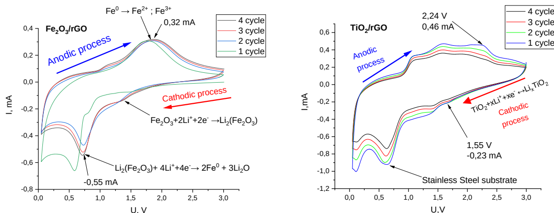
Figure 4.4. CV curves of the first four cycles of \text{Fe}_2\text{O}_3/\text{rGO} and \text{TiO}_2/\text{rGO} . Voltage sweep rate 1 \text{ mVs}^{-1} , voltage range 0.05\text{--}3 \text{ V} .
