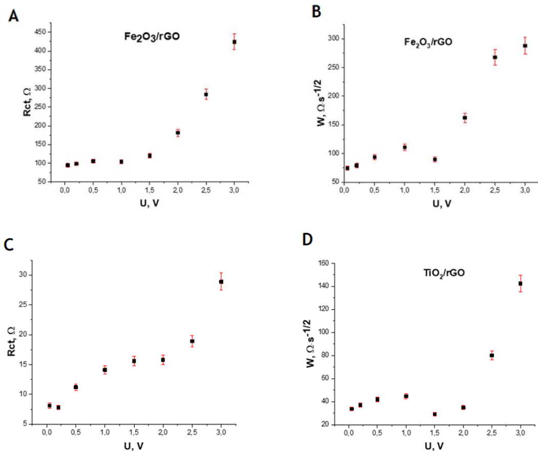
Figure 4.5. Fe 2 O 3 /rGO and TiO 2 /rGO electrode material charge transfer resistance (A, C) and Warburg impedance (B, D) as a function of battery half-cell voltage.
