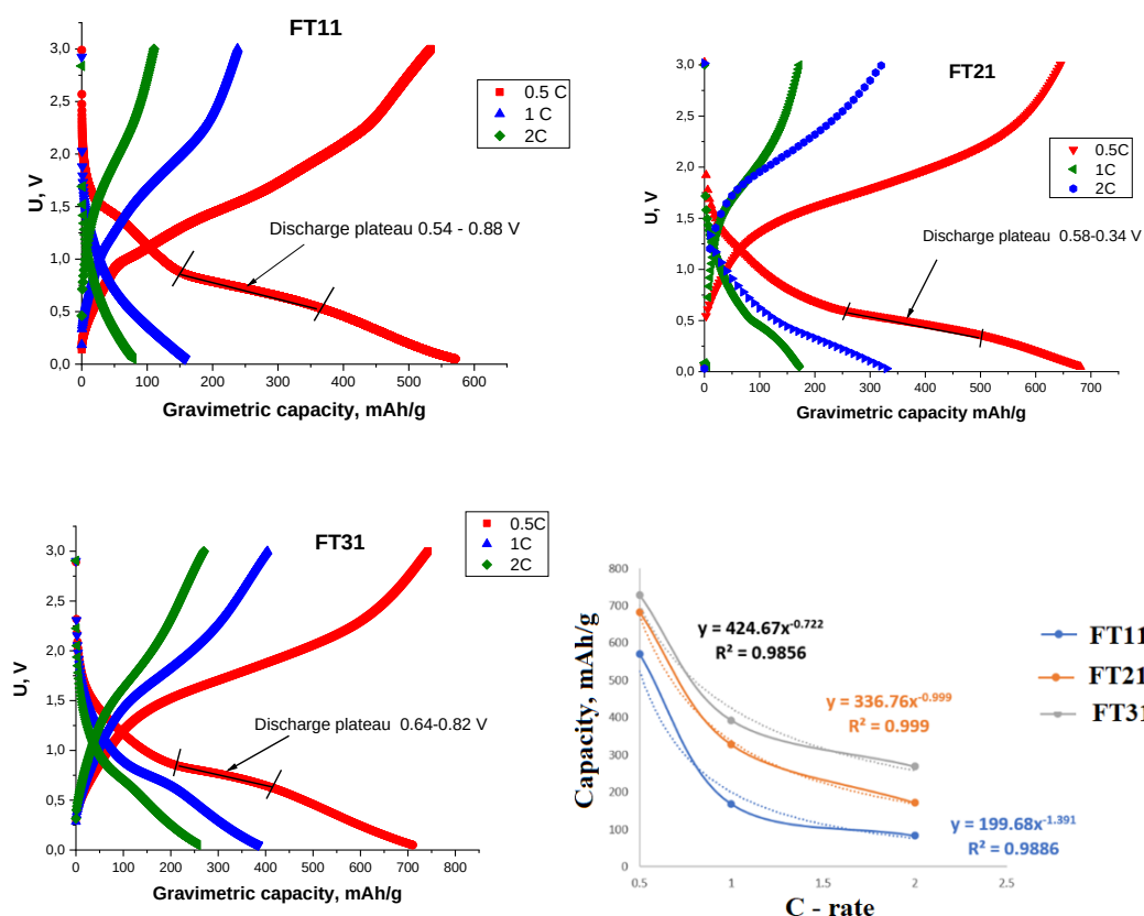
Figure 4.9. Galvanostatic charge-discharge curves of FT11, FT21 and FT31 nanocomposite electrodes taken at current strengths of 0.5C, 1C and 2C and charge capacity as a function of discharge current.
