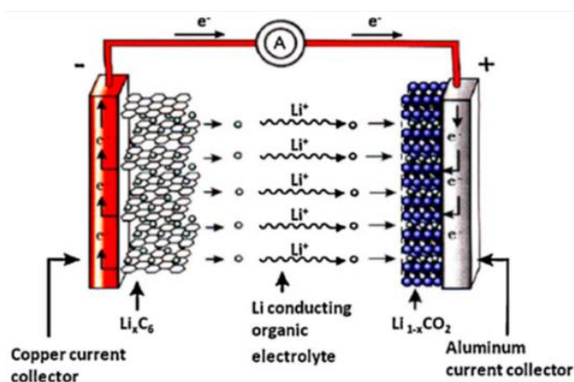
Figure 2.1. Simplified battery discharge process [2]
