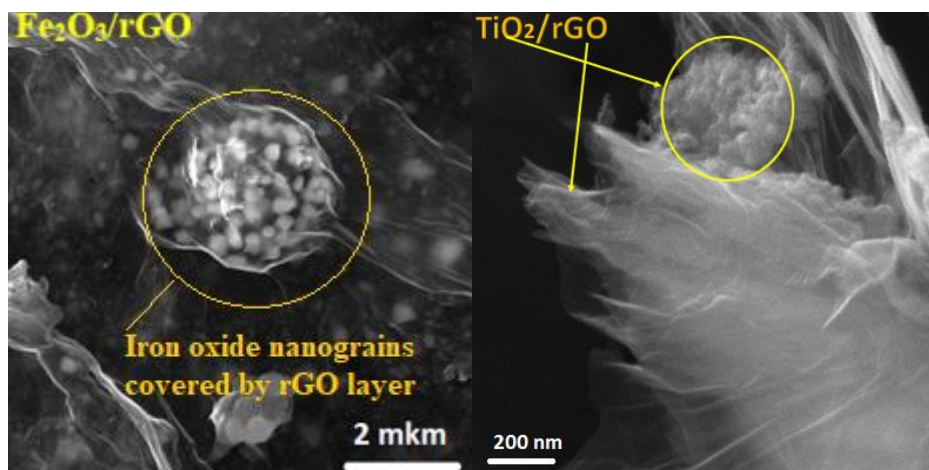
Figure 4.1. SEM images of \text{Fe}_2\text{O}_3/\text{rGO} and \text{TiO}_2/\text{rGO} layers.
