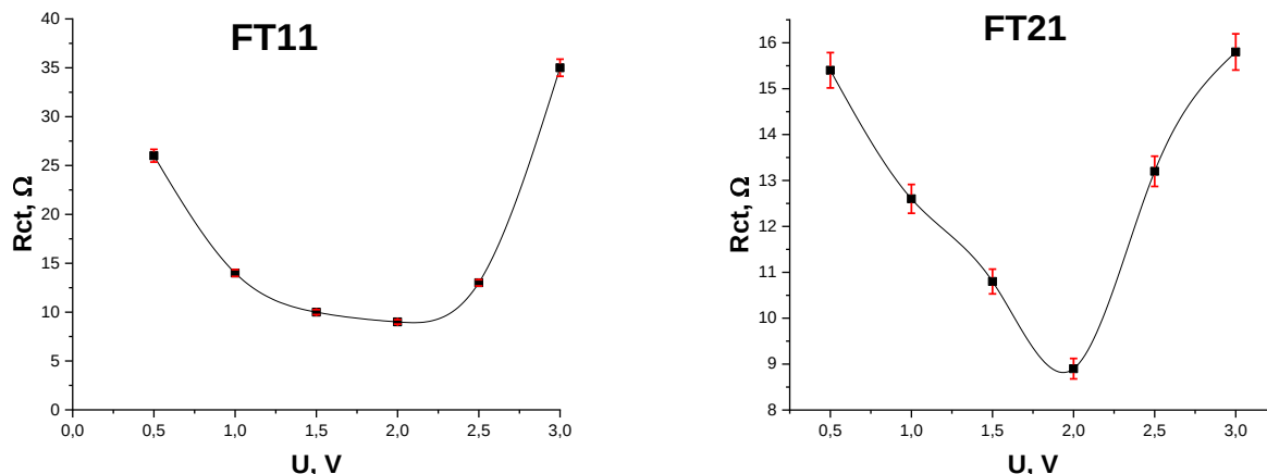
Figure 4.13. Charge transfer resistance as a function of the state of charge of the battery half-cell.
