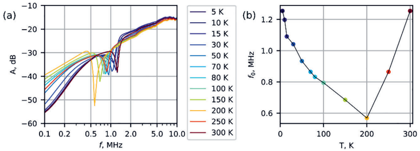
Figure 4.3. Vibration dependence on temperature for a \text{Bi}_2\text{Se}_3 nanobelt. (a) S21 amplitude parameter for a \text{Bi}_2\text{Se}_3 nanobelt as a function of temperature in range 5–300 K. (b) Dependence of negative peak frequency f_0 on temperature shows more than a twofold decrease of resonant frequency when the temperature is increased from 5 K to 200 K
