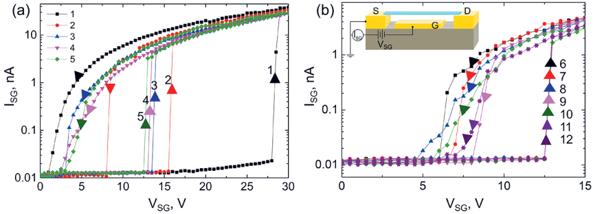
Figure 4.11. Switching characteristics of an integrated CuO NEM switch during the initial cycles. (a) V_{\text{ON}} changes gradually from 28.0 V (black curve) to 12.5 V (green curve) during the first five cycles of operation. (b) Following the first cycles, a regime with constant V_{\text{ON}} of 12.5 V is established
