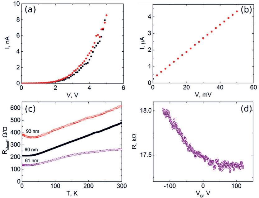
Figure 4.4. Contact optimization and charge transport properties of Bi _2 Se _3 nanobelts. Contact optimization using wet etching allowed to change I-V characteristics from non-linear with high resistance (a) to linear with low resistance (b). (c) Temperature dependence of sheet resistance for 3 suspended nanobelts with different thicknesses in temperature range from 300 K to 2 K. (d) Resistance dependence on gate voltage at 2 K points to n-type majority charge carrier field-effect
