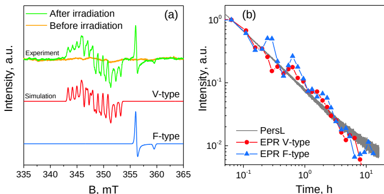
Fig. 4.9. (a) EPR spectra of the x = 0.10 mol% \text{Cr}^{3+} sample before and after UV irradiation; (b) EPR signal intensity decay compared to PersL decay kinetics.
