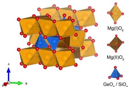
Fig. 2.2. Crystal structure of \text{Mg}_2\text{SiO}_4 and \text{Mg}_2\text{GeO}_4 and polyhedron of \text{Mg}^{2+} , \text{Si}^{4+} and \text{Ge}^{4+} .
