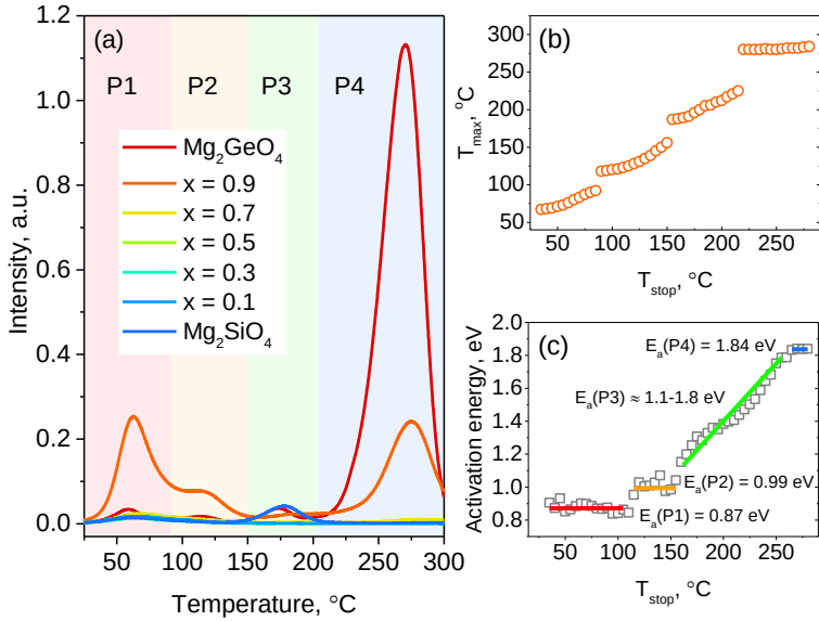
Fig. 4.14. (a) TSL glow curves of the MSGO samples after irradiation with 263 nm; (b) T_{\text{max}} - T_{\text{stop}} plot; (c) E_a - T_{\text{stop}} plot.
