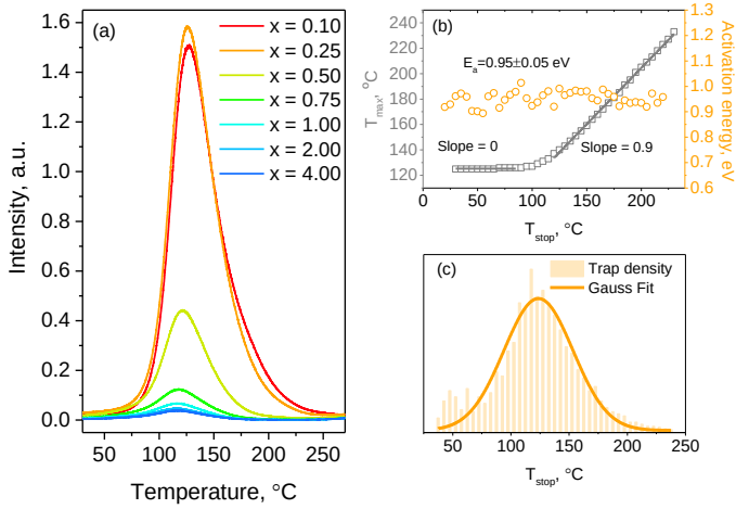
Fig. 4.8. (a) TSL glow curves of the MGO samples after irradiation with 263 nm; (b) T_{\max} - T_{\text{stop}} plot and E_a values; (c) the calculated trap density distribution.
