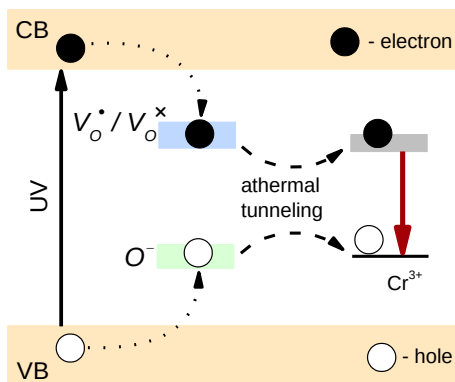
Fig. 4.10. A schematic diagram of the PersL mechanism in the MGO material.
