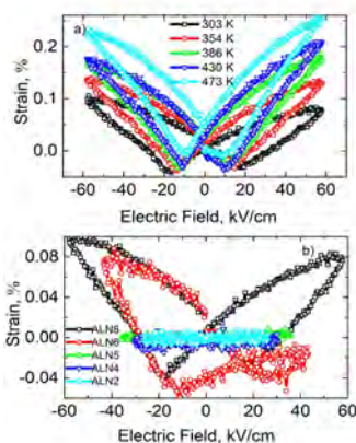
Fig.1.D(E) a) for \text{ALN}_6 at different temperatures; b) for ALN at different lithium concentrations.
