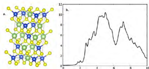
Fig. 1 a. – chalcopyrite crystal structure, b. – example of calculated spectra (CuGaS 2 )
