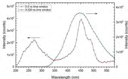
Emission spectra of BaGeF 6 in two time windows, 0-3 ns and 3-320 ns.
