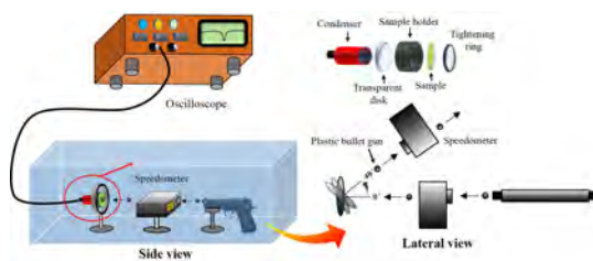
The schematic illustration of self-designed I-ML measurement setup.
