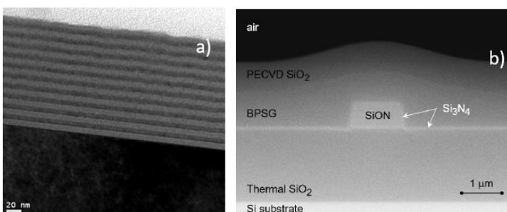
High resolution TEM cross section of a annealed Si/SiO 2 multilayer, b) SEM cross-section of a SiON waveguide
