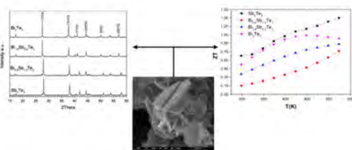
Nanostructured Bi 2-x Sb x Te 3 materials, structure, morphology and thermoelectric figure of merit.
